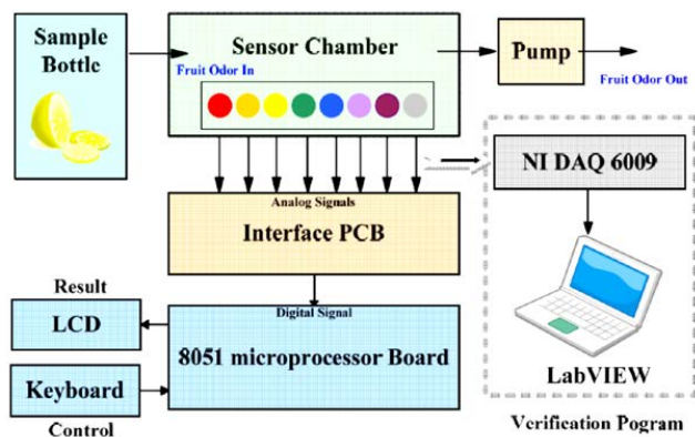
Fig. 2. Block diagram of e-nose system [22]
