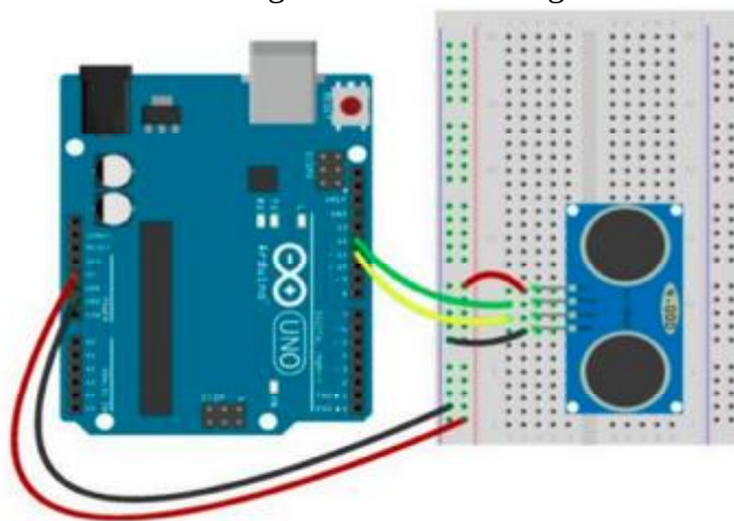
Fig. 2. Connection diagram of the sensor HR-SR04 on the Arduino microcircuit board
