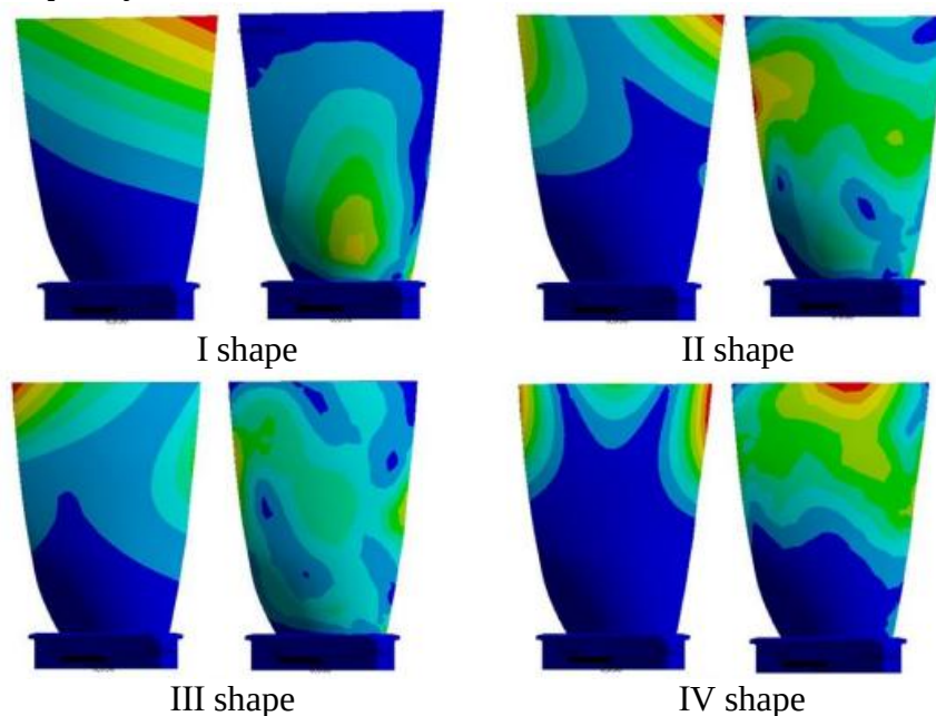
Fig. 1. Displacement patterns (left) and relative stresses (right) for the blade of the first stage
