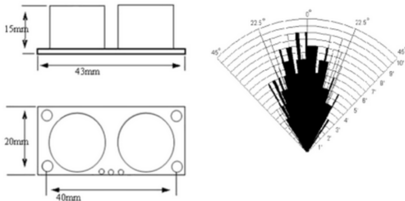
Fig. 1. Directional diagram
