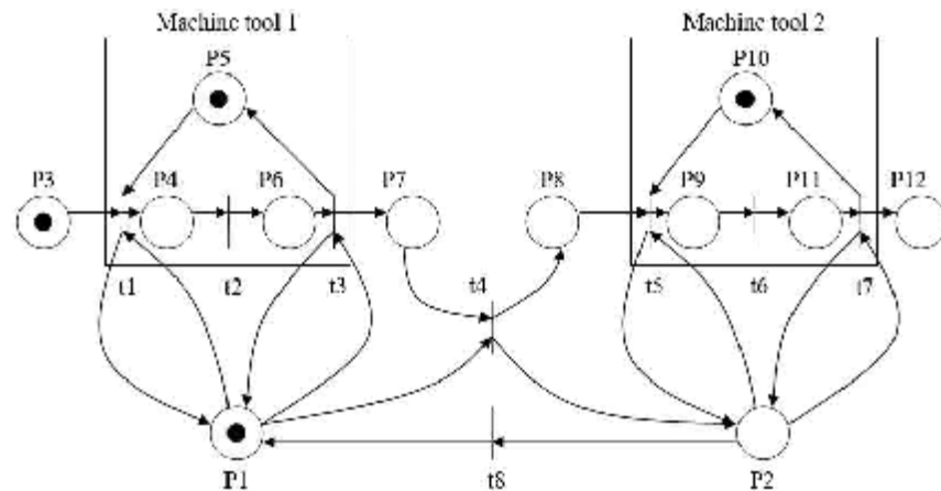
Fig. 2. A two-station system with an attendant robot described by a Petri net
