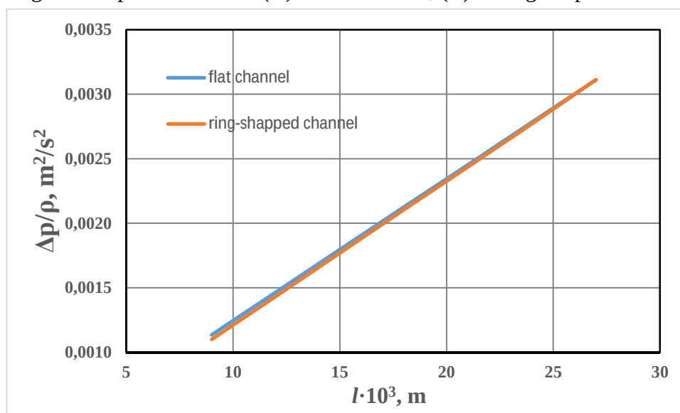
Fig. 2. The pressure drops versus the channel length
