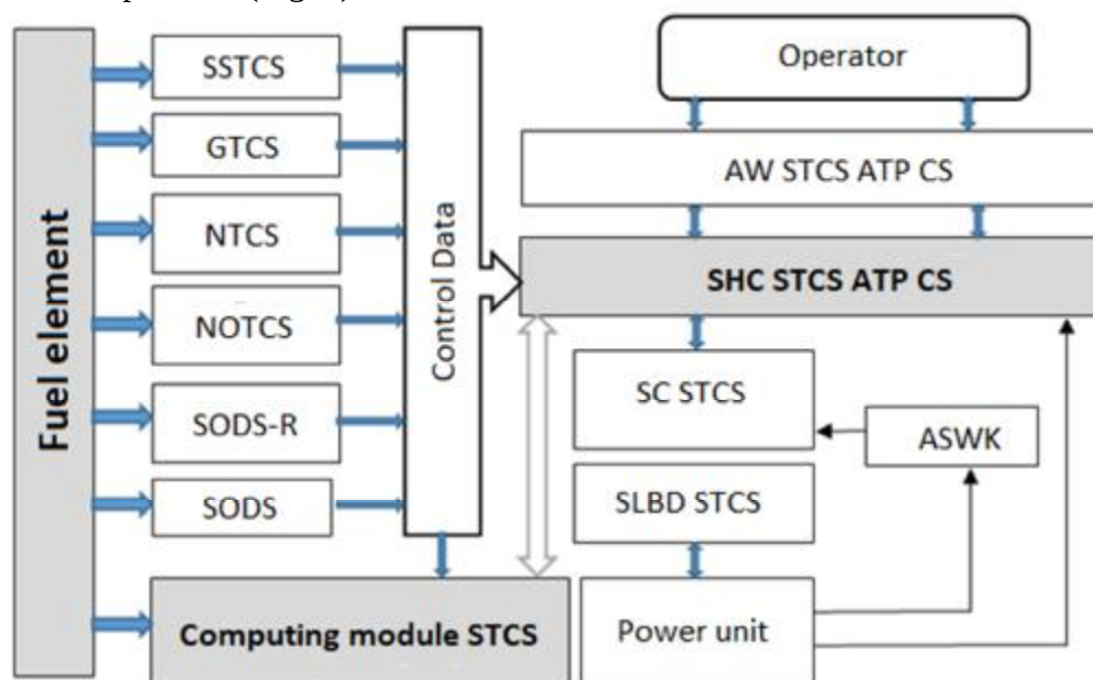
Fig. 1. Improved structural and functional system of the shell of the fuel element of the nuclear reactor tightness control system.
