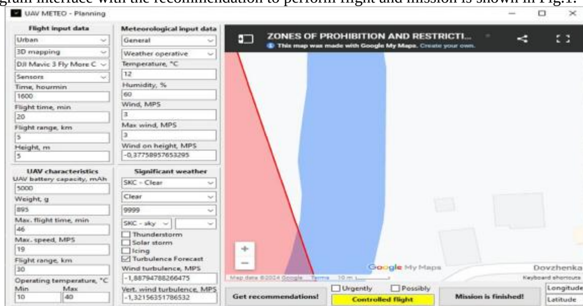
Fig. 1. UAV METEO program interface
