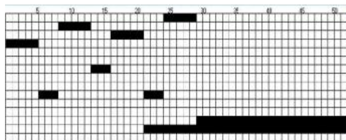
Fig. 3. Cycle diagram of operation of the robot of the two-station system
