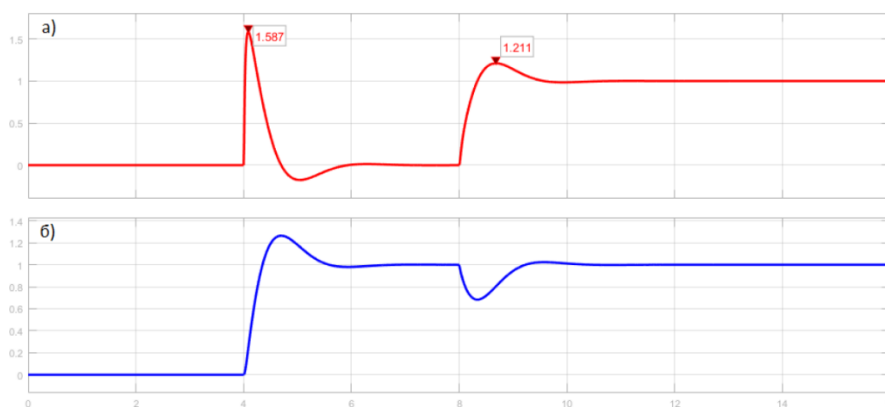
Fig. 2. Time-domain characteristics of torque and speed with the sensor
