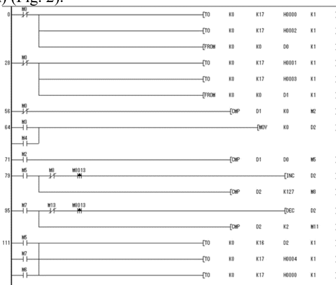
Fig. 2. GFR operation program in Ladder Diagram language
