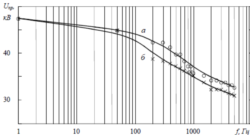
Fig. 2. Dependence of breakdown voltage on high voltage frequency for telephone wire KSPV 4 0.12 (a) and LAN cable KSSPV UTP 4 Cat. 5e (b) wires
