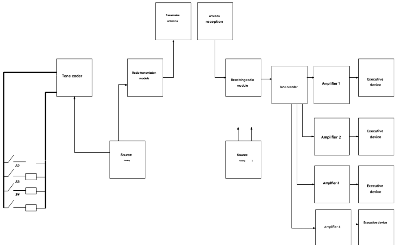
Fig. 3. Block diagram of the servo drive control unit (wireless device)
